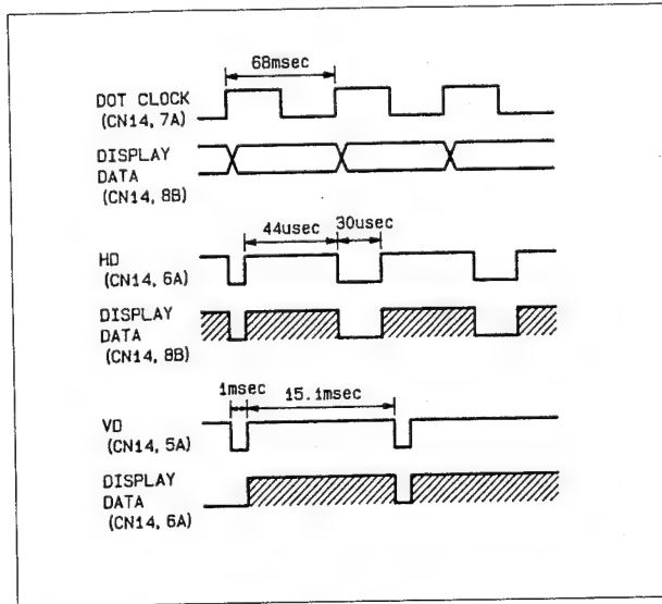
Fig. 6-4-1. Timing Chart (EL Display)
